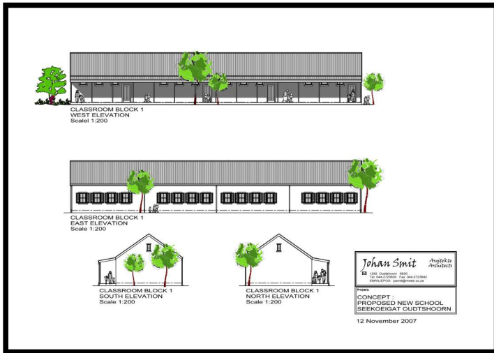
Block 1 - Elevation
