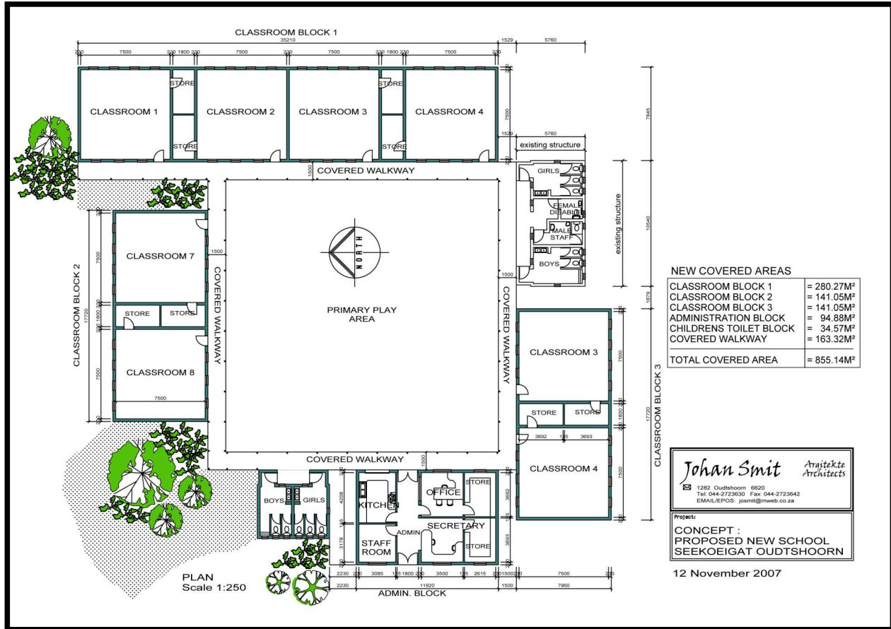
Zeekoegat Primary School - Plan with COVERAGE
