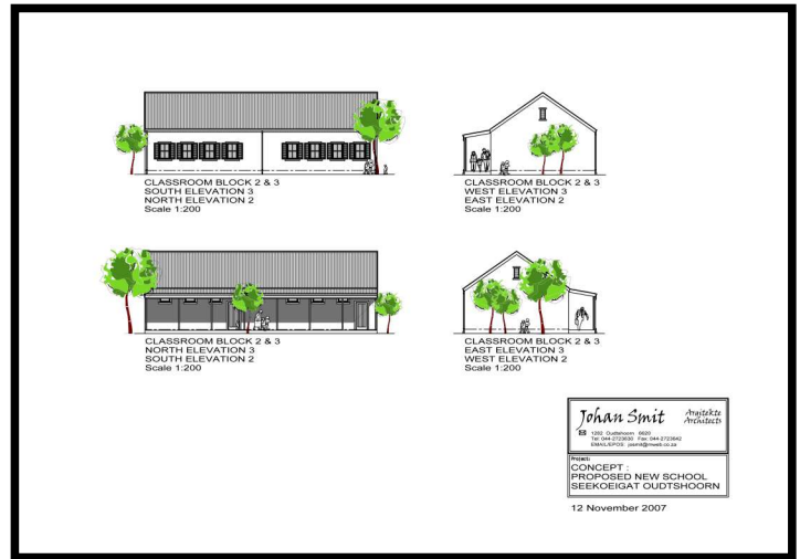
Block 2 & 3 - Elevation
