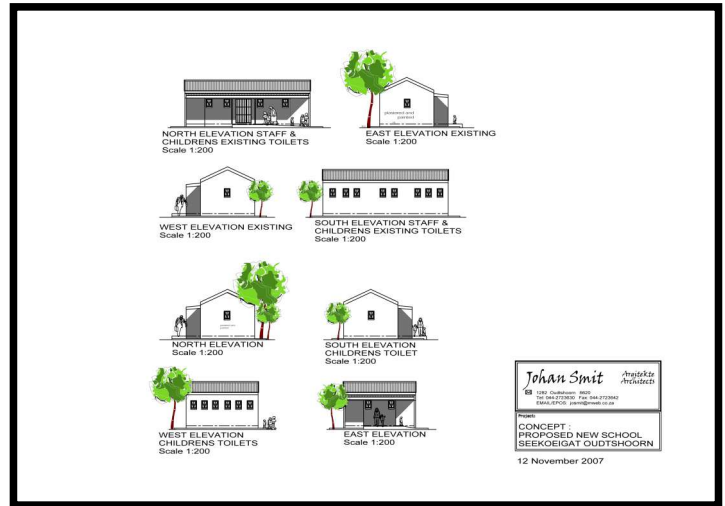
Toilets - Elevation
