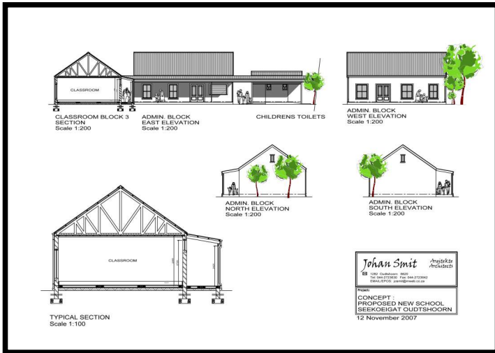
Aministration - Elevation
